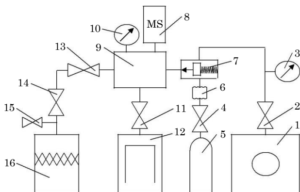
Fig. 1 – Schematic diagram of the UVBL-4 vacuum unit: 1 – mechanical pre-vacuum pump; 2, 4 – shut-off valves; 3 – manometric transducer PMT-4M; 5 – cylinder with reference gas; 6 – bypass cylinder; 7 – dosing valve; 8 – analyzer of mass spectrometer MX7304; 9 – vacuum chamber; 10 – manometric transducer PMM-32; 11 – high vacuum valve DU-50; 12 – magnetic discharge pump NMDO-0.25; 13, 14 – shut-off valve DU-12; 15 – safety valve; 16 – adsorption coal pump
