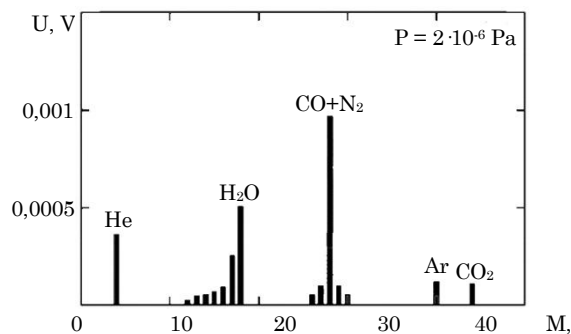
Fig. 2 – Mass spectrum of the residual atmosphere of the vacuum chamber at a rarefaction in it of 2 \cdot 10^{-6} Pa
