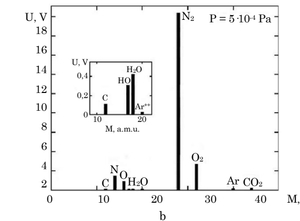
Fig. 4 – Mass spectra of the gaseous environment: from the zones of AEW (a) and ESA (b) when inlet into the vacuum chamber to pressure 5 \cdot 10^{-4} Pa
