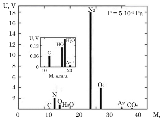
Fig. 3 – Mass spectrum of clean air when it is admitted into a vacuum chamber up to a pressure of 5 \cdot 10^{-4} Pa
