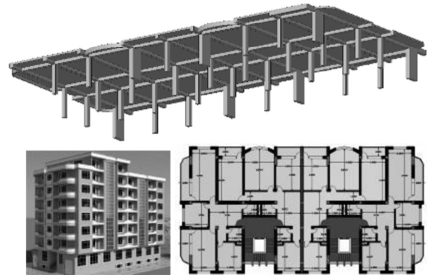
Figure 1 The physical model of the fragment of a monolithic overlapping of a residential house in the Sumy (a); 3d model of a living skeleton house (b); typical floor plan (c)
