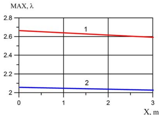
Figure 4 – Calculated dependence of the Mach number M (1) and the relative velocity of the gas stream \lambda (2) along the length of the tubular guide at the moment the projectile leaves the guide (the flow moves from right to left)
