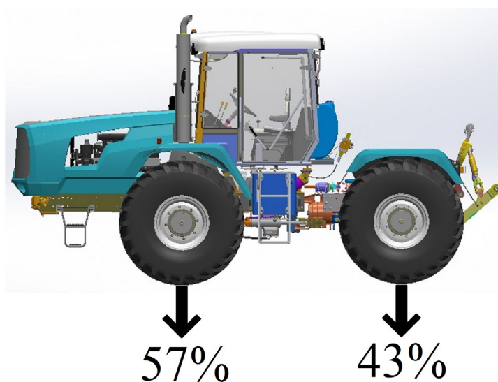
Figure 1 – Layout of the 4K4b tractor produced by JSC "KhTP" with indication of the percentage of the mass distributed on the axles
