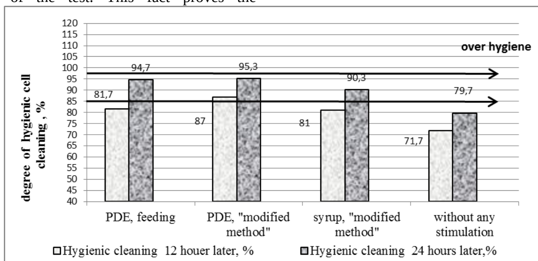
Fig. 2. Evaluation of hygienic cleaning of bee colonies by the «perforation test» in different methods of PDE application
