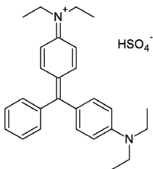
Fig. 3. Structure of Brilliant Green
