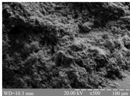
Fig. 11. Fungus mycelia in concrete (scanning electron microscopy)
