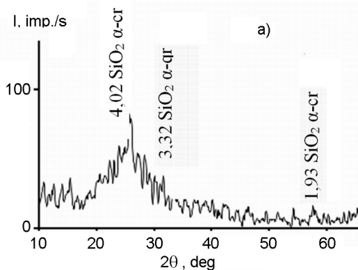
Fig. 3. X-ray patterns of quartz ceramics without additive (a) and with modifying additive in the amount of 1.5 wt.% (b): cr — cristobalite, qr — quartz.
