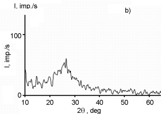
Fig. 3. X-ray patterns of quartz ceramics without additive (a) and with modifying additive in the amount of 1.5 wt.% (b): cr — cristobalite, qr — quartz.
