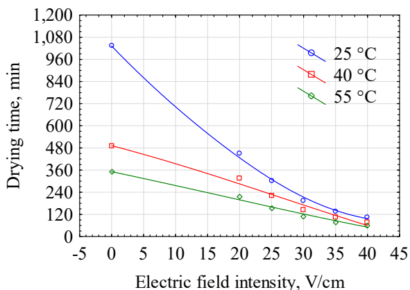
Fig. 3. Dependence of drying time on the intensity of a direct electric heating field at an air temperature in the dryer of 25, 40, and 55 °C
