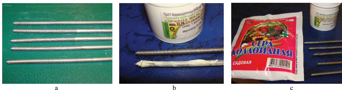
Fig. 1 – The electrodes are made of 12X18H10T (12H18N10T) stainless steel Ø 3mm intended for sulphiding the parts by EEA method
